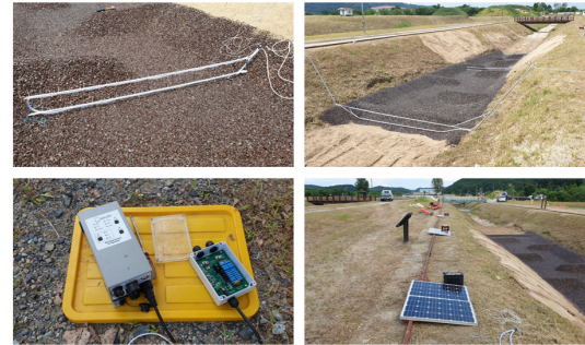
Fig. 5. Installation of pit-tag antenna, sensor module, and solar rechargeable battery.
